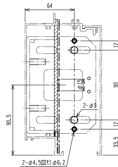
Comfort N 100見込 (複層)
