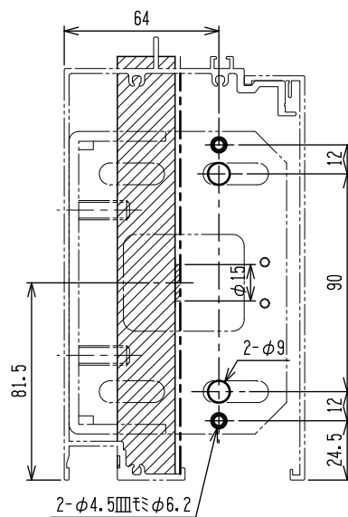
Comfort N 100見込 (単板)
